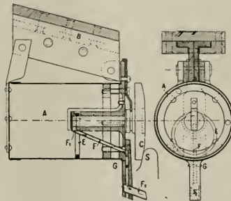
DETAILS OF MONTRÉUX-OBÉRLAND FLANGE LUBRICATION
